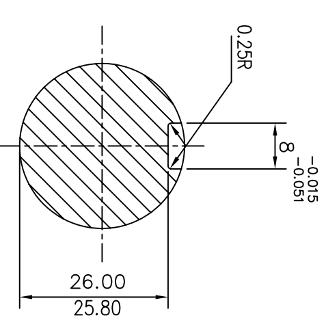
KEYWAY DETAIL (INPUT) --R14:R18:1
